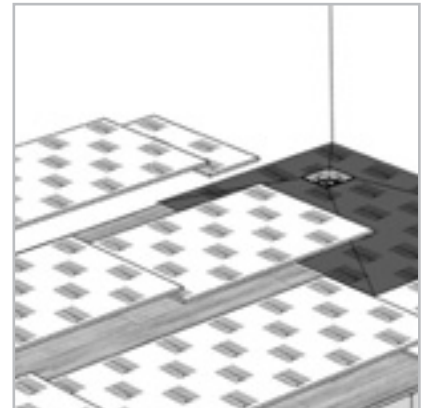
Floor leveling with shower base flush with the floor
